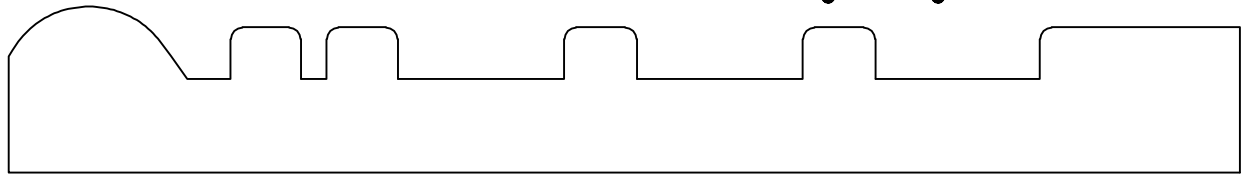
B-824 3/4" X 6 1/2"
