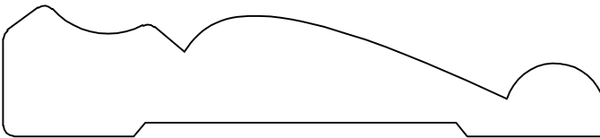
B-856 \frac{3}{4}" \times 3\frac{1}{2}"
