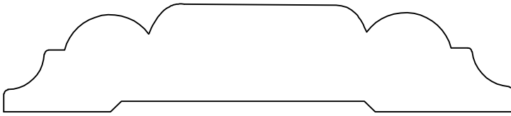
B-846 7/8" X 3 3/4"
