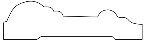
B-834 3/4" X 2 1/2"
