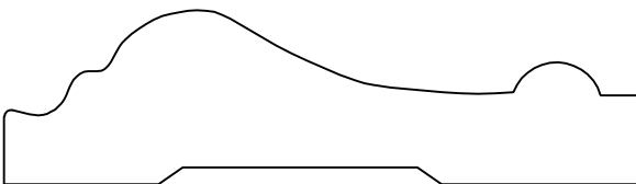
B-860 \frac{3}{16}" \times 3"
